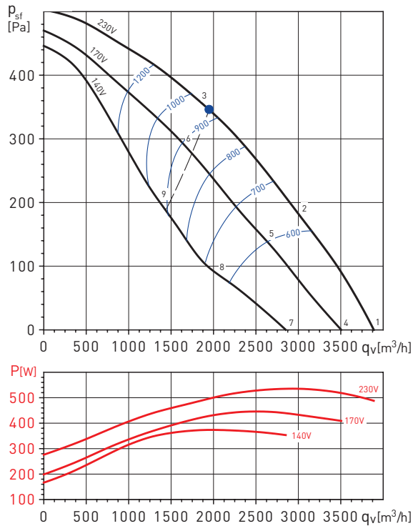
VENT-400N
